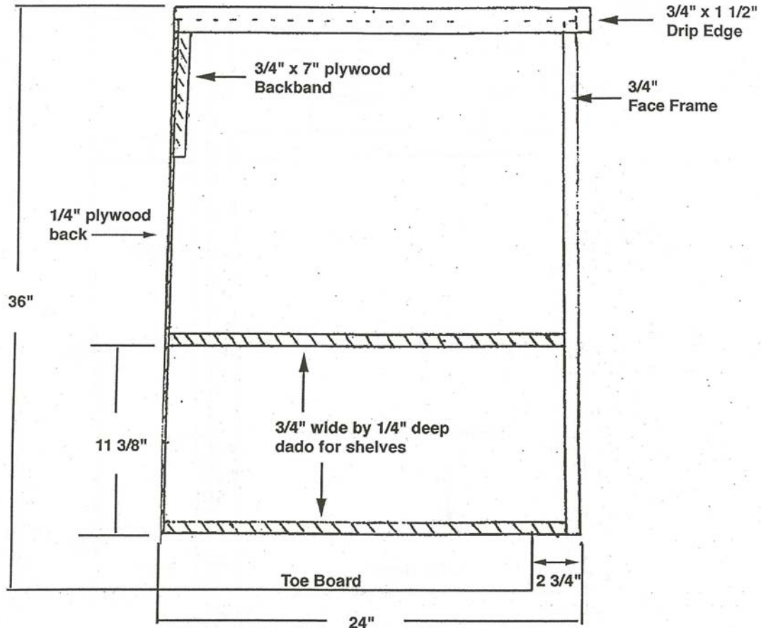
Base Cabinet Side View
