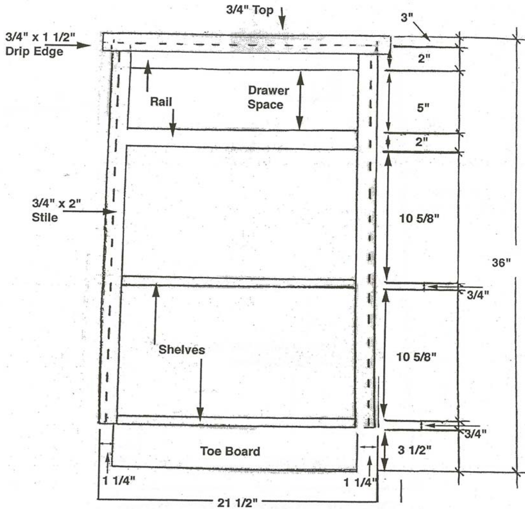
Base Cabinet Front View
