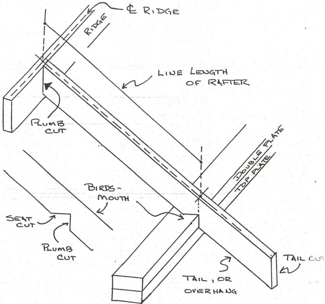
FIG. 3 PARTS OF A RAFTER
