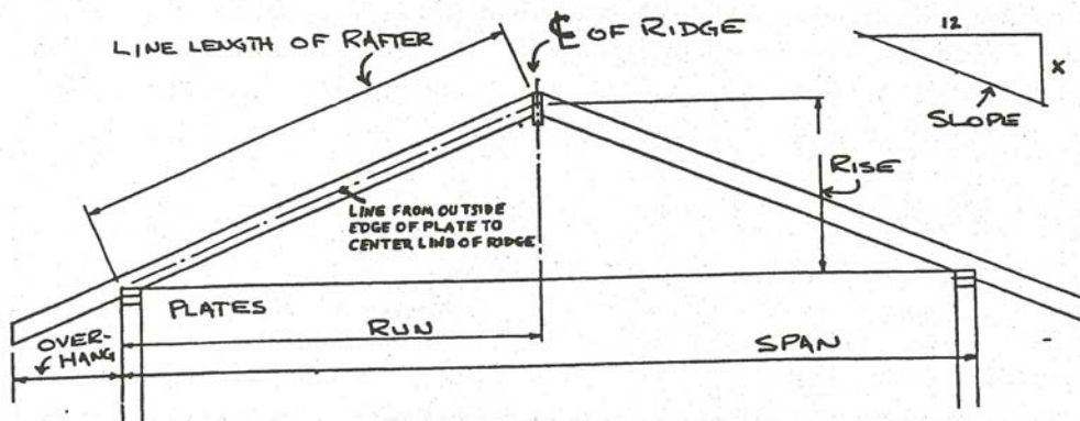
FIG. 5 BASIC TERMS AND DIMENSIONS USED IN RAFTER LAYOUT.
