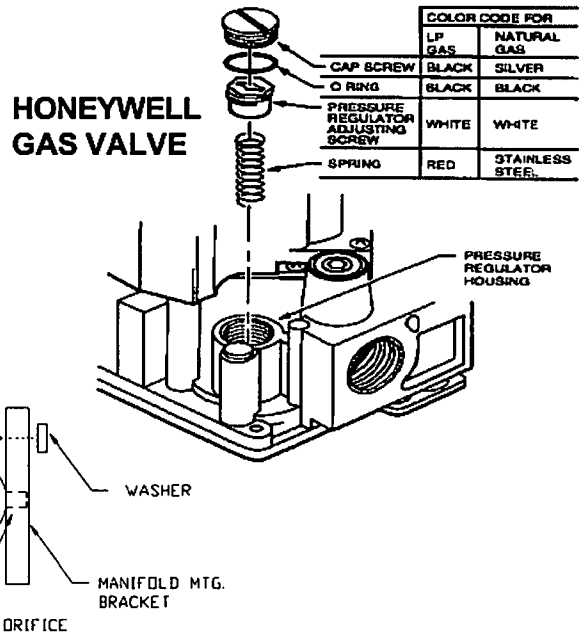
FIGURE 4 GMPN FURNACE ONLY (SHOWN IN UPFLOW POSITION)
